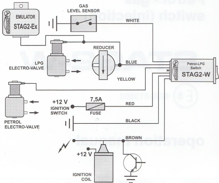
Fig.1. Connection diagram
